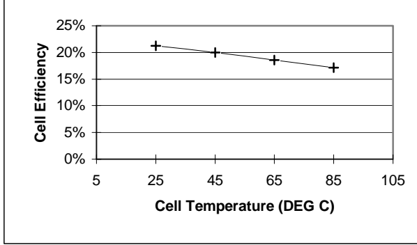
Figure 4 A: One-Sun Efficiency of AMNX 1805 as a Function of Temperature
