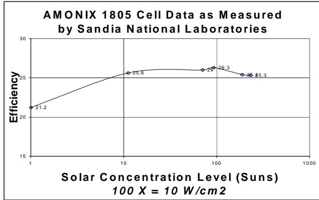
Figure 5: AMNX 1805 Efficiency Data
